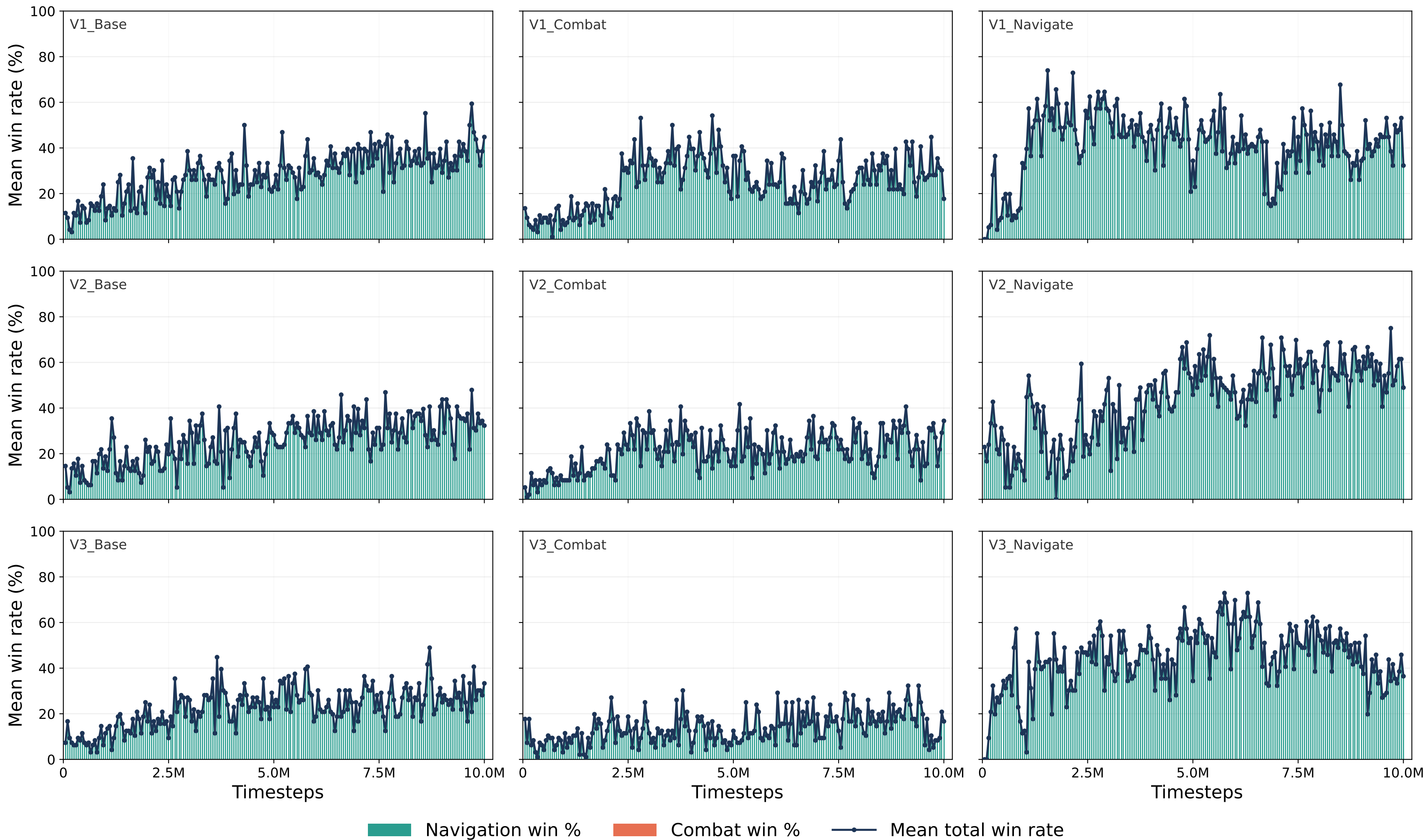
MaskPPO mean stacked win conditions by map variant
